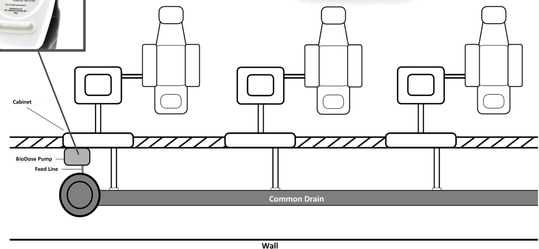
AERIAL VIEW OF A DIALYSIS DRAIN SYSTEM
